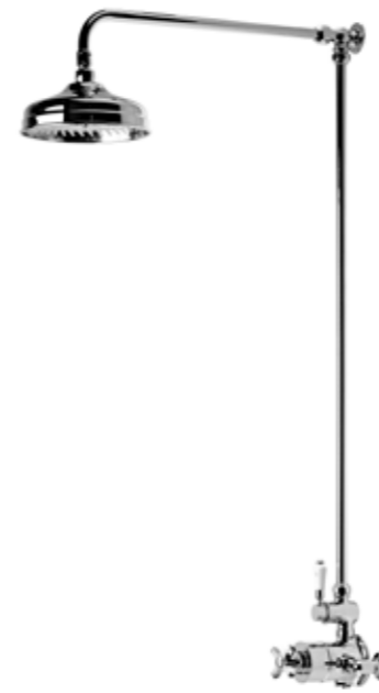
Wessex single function shower system with overhead shower • Thermostatic sequential shower valve • Height adjustable rigid riser rail with flow control to overhead shower • Overall system height 1110mm, rigid riser rail can be cut to height • 200mm brass shower head Min pressure 0.3bar
